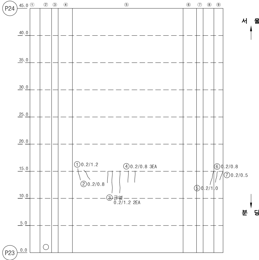
KEY PLAN
